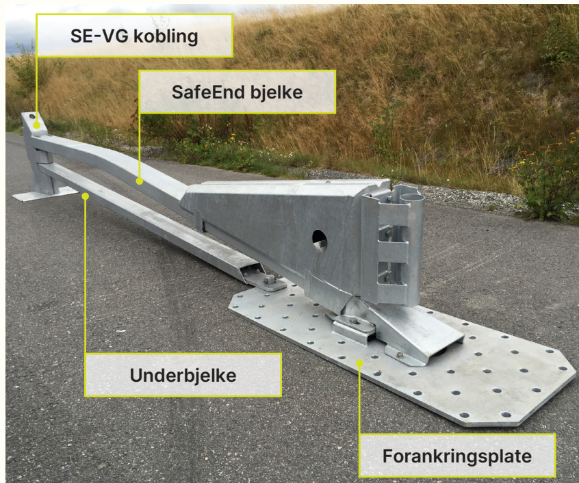
SafeEnd 80T-NO: LxB 5.2m x 0.25 m
